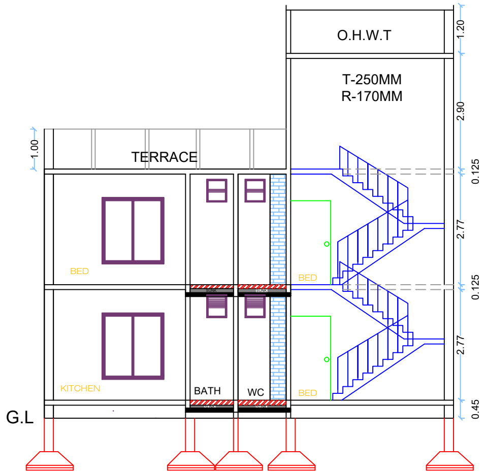
SECTION-AA'
