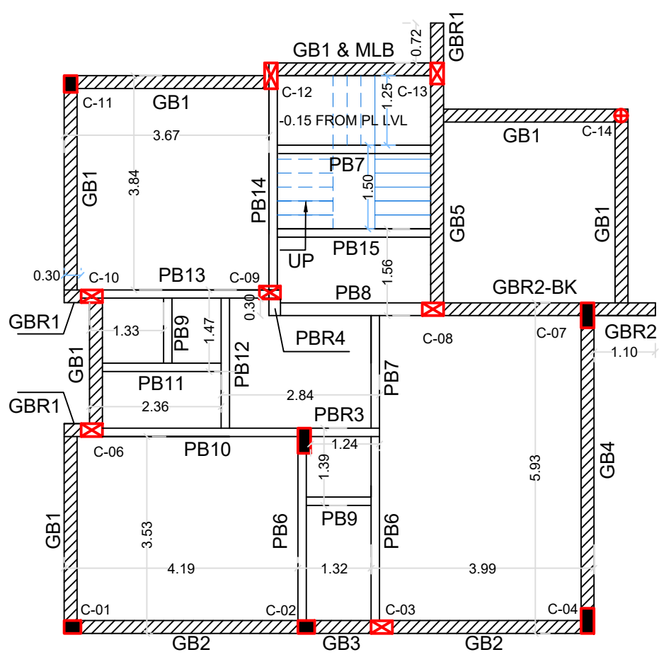
BEAM LAYOUT AT PLINTH LEVEL
