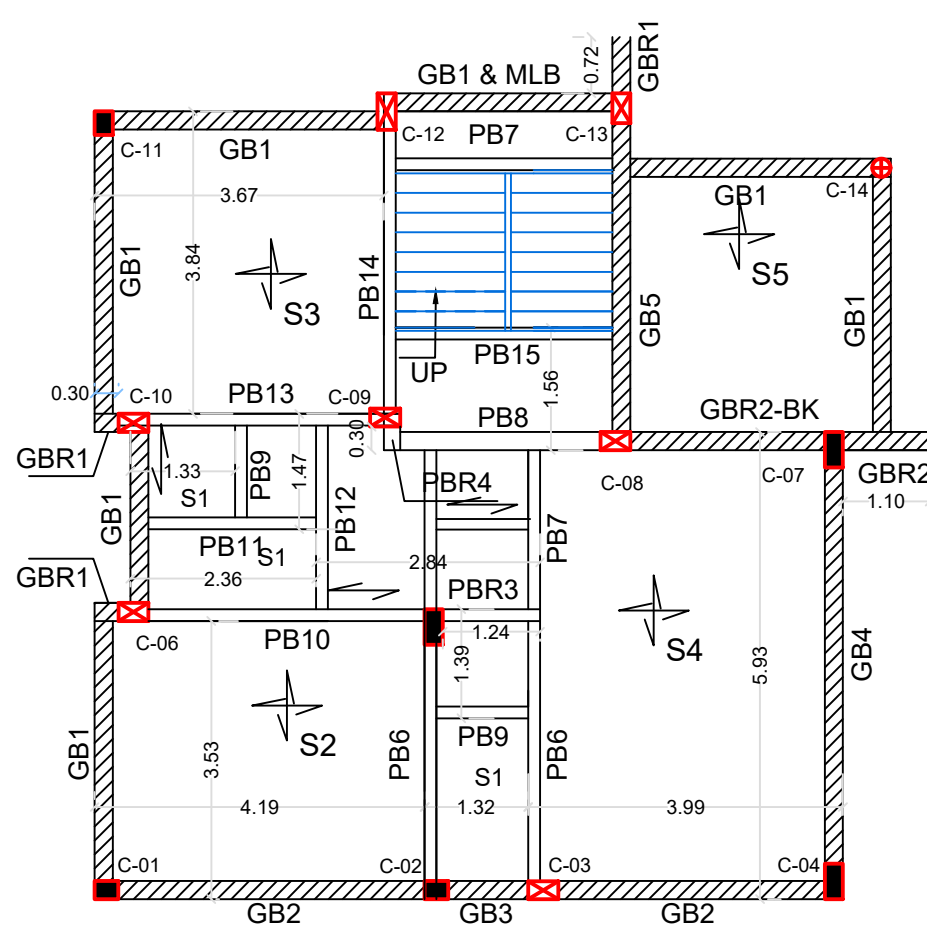
BEAM AND SLAB LAYOUT AT GROUND LEVEL
