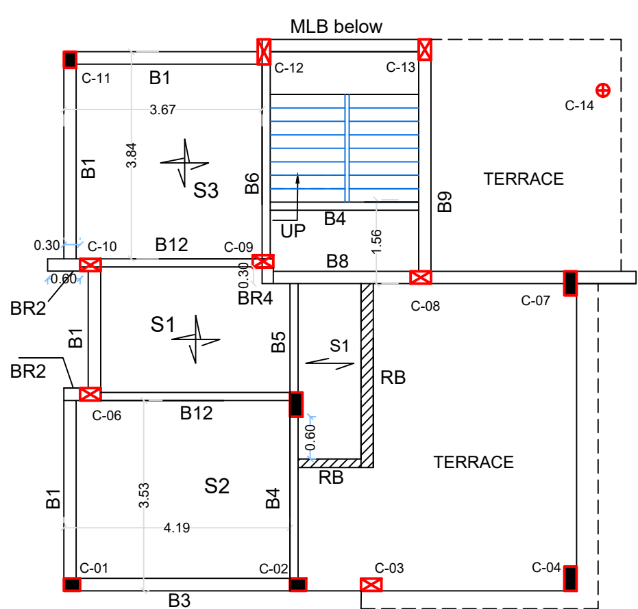
BEAM AND SLAB LAYOUT AT TERRACE LEVEL
